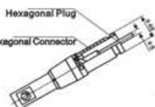
STRUCTURE OF HEXAGONAL PLUG
