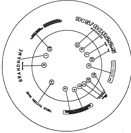
LOWER MOLD
