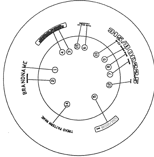
UPPER MOLD
