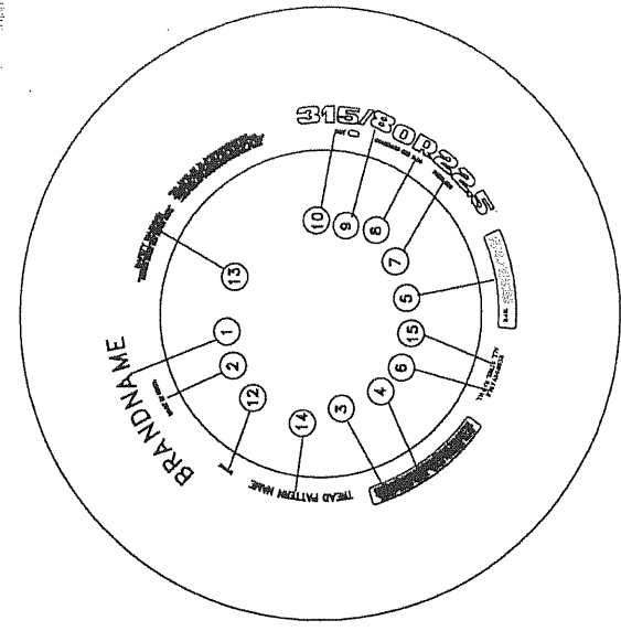
UPPER MOLD
