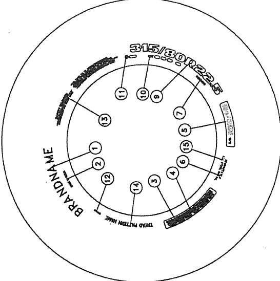
LOWER MOLD
