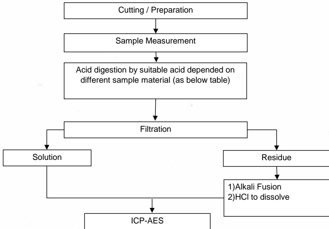
Method 1: Flow Chart of Digestion for Cd analysis
