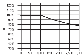
4) Derating chart
