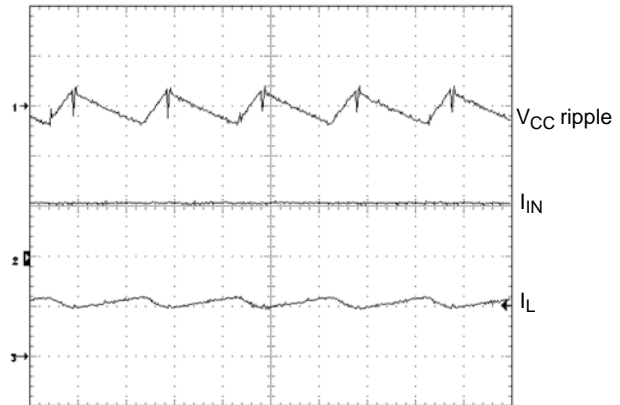
Figure 7. Boost Input Voltage and Current Ripple Waveforms
