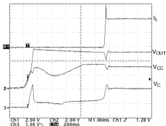
Figure 4. Startup Waveforms of Circuit Shown in the Application Diagram.
