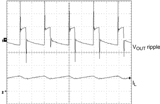
Figure 9. Typical Output Voltage Ripple
