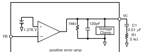
Figure 3. Error Amplifier Equivalent Circuit
