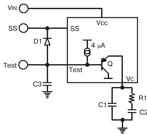
Figure 13. Soft Start
