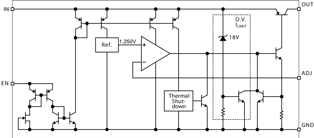
* LM39302 Adjustable Output with Enable
