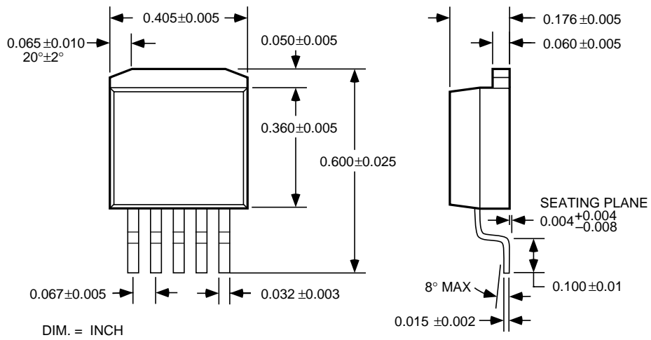
5-Lead TO-263-5 (S)
