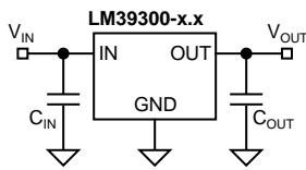
Figure 1. Capacitor Requirements
