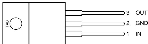
LM39300-x.xBT TO-220-3 (T)
