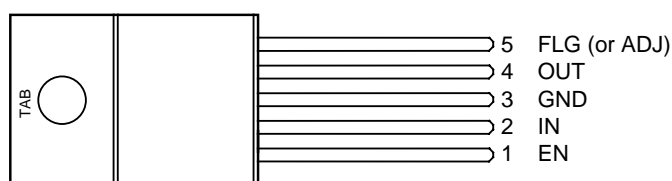
LM39301-x.x, LM39302BT TO-220-5 (T)
