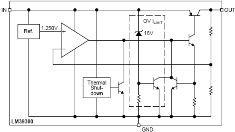
* LM39300 Fixed output (1.5V, 1.8V, 2.5V, 3.3V, 5.0V)
