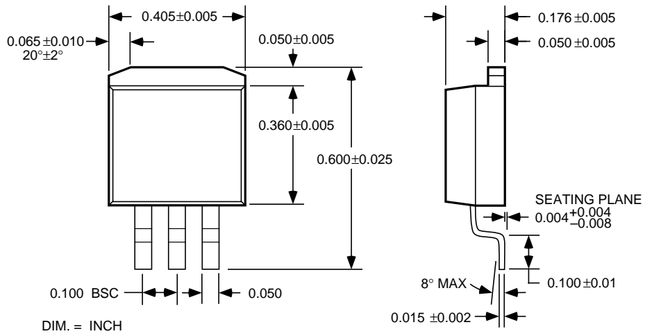
3-Lead TO-263 (S)
