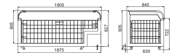
封头柜/Terminal cabinet
