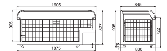
封头柜/Terminal cabinet
