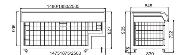
直柜/Direct cabinet
