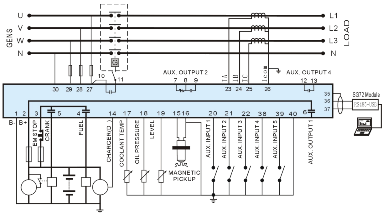
HGM6110UC Typical Application Diagram
