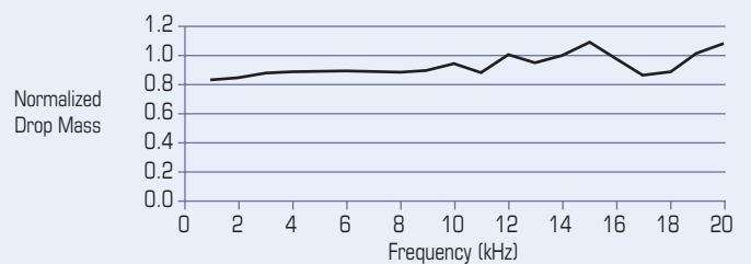
Galaxy 30 AAA Drop Mass Frequency Response
