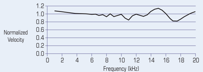
Galaxy 30 AAA Velocity Frequency Response
