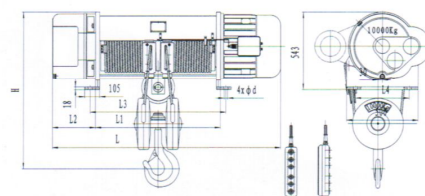
CD/MD, 型固定式10吨 (H=9-30米) Model CD 1 /MD 1 Stationary 10t (H=9-30m)
