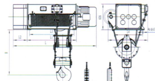
WH164型固定式20吨 (H=9-30米) Model WH164 Stationary 20T(Hoisting 9-30m)
