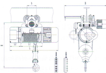
CD/MD, 型0.25-5吨 (H=6-9米) Model CD 1 /MD 1 0.25-5t (H=6-9m)
