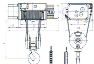
WH164型固定式32吨 (H=9-24米) Model WH164 Stationary 32T(Hoisting 9-24m)
