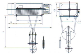
WH164型固定式16吨 (H=12-48米) Model WH164 Stationary 16T(Hoisting 12-48m)
