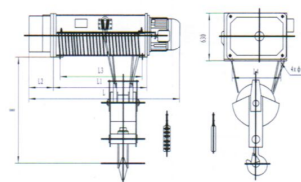
WH164型固定式20吨 (H=9-24米) Model WH164 Stationary 20T(Hoisting 9-24m)
