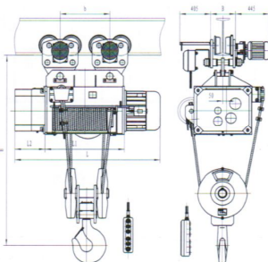
WH164型32吨 (H=9-24米) Model WH164 32T(Hoisting 9-24m)
