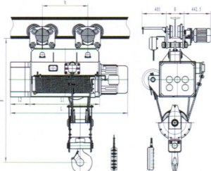
WH164型20吨 (H=9-30米) Model WH164 20T(Hoisting 9-30m)
