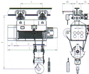
WH164型16吨 (H=9-36米) Model WH164 16T(Hoisting 9-36m)
