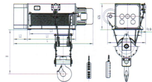
WH164型固定式16吨 (H=9-36米) Model WH164 Stationary 16T(Hoisting 9-36m)
