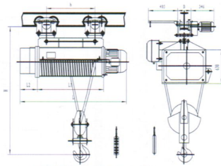
WH164型16吨 (H=12-48米) Model WH164 16T(Hoisting 12-48m)
