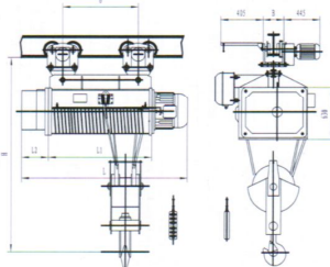
WH164型20吨 (H=9-24米) Model WH164 20T(Hoisting 9-24m)
