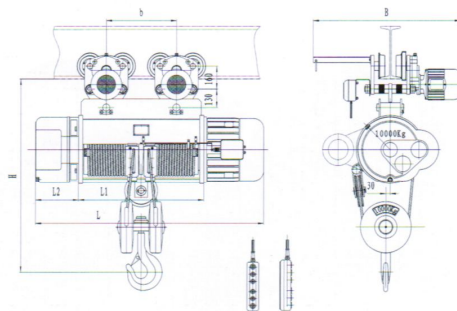
CD/MD, 型10吨 (H=9-30米) Model CD 1 /MD 1 10t (H=9-30m)
