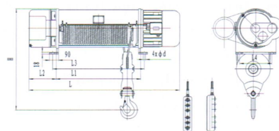
CD/MD, 型固定式0.5-5吨 (H=12-30米) Model CD 1 /MD 1 Stationary 0.5-5t (H=12-30m)
