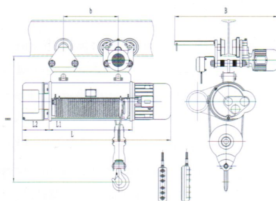
CD/MD, 型0.5-5吨 (H=12-30米) Model CD 1 /MD 1 0.5-5t (H=12-30m)
