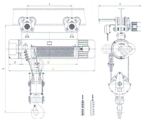
CD/MD, 型16吨 (H=9-30米) Model CD 1 /MD 1 16t (H=9-30m)
