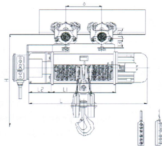
HB型 10吨(H=9-30米) Model HB 10T(H=9-30m)
