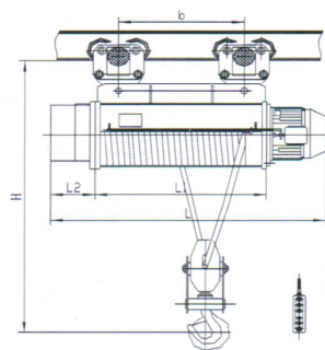
HB型 16吨(H=12-48米) Model HB 16T(Hoisting 12-48m)
