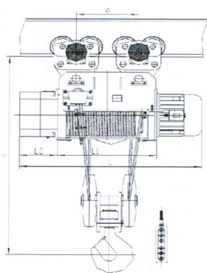
HB型 32吨(H=9-24米) Model HB 32T(Hoisting 9-24m)
