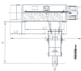
HB型固定式 20吨(H=9-24米) Model HB Stationary 20T (Hoisting=9-24m)
