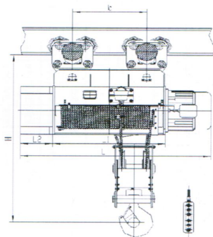
HB型 20吨(H=9-24米) Model HB 20T(Hoisting=9-24m)
