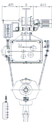
HB, 型 16吨(H=9-36米), 20吨(H=9-30米) Model HB, 16T(Hoisting 9-36m), 20T(Hoisting 9-30m)
