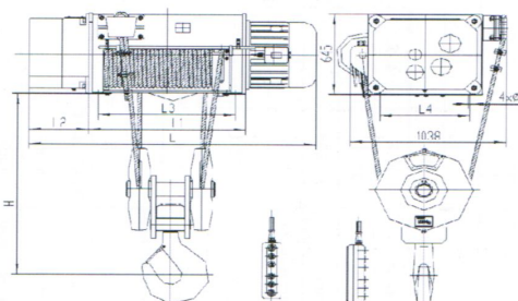
HB型固定式 32吨(H=9-24米) Model HB Stationary 32T(Hoisting 9-24m)
