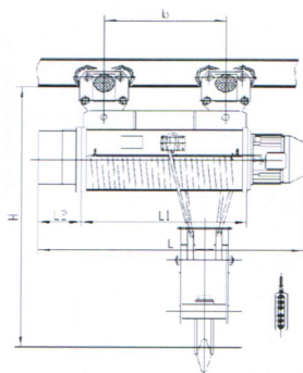
HB型 20吨(H=9-24米) Model HB 20T(Hoisting=9-24m)
