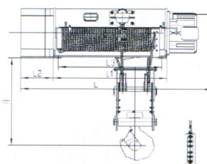
HB, 型固定式 16吨(H=9-36米), 20吨(H=9-30米) Model HB, Stationary 16T(Hoisting 9-36m), 20T(Hoisting 9-30m)
