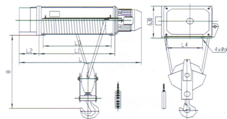
HB型固定式16吨(H=12-48米) Model HB Stationary 16T(Hoisting 12-48m)
