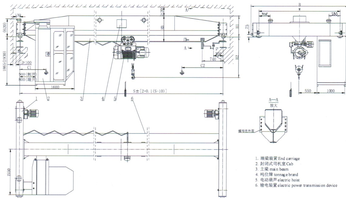
外形结构图 (安装有机室) Exterior structure diagram (with operation room)
