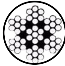
7 x 7
