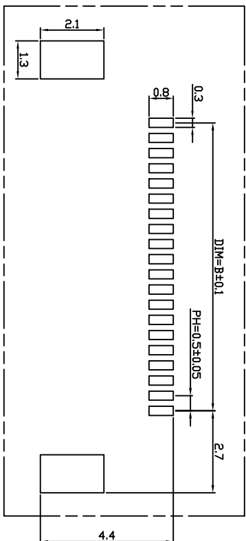
PCB Layout
