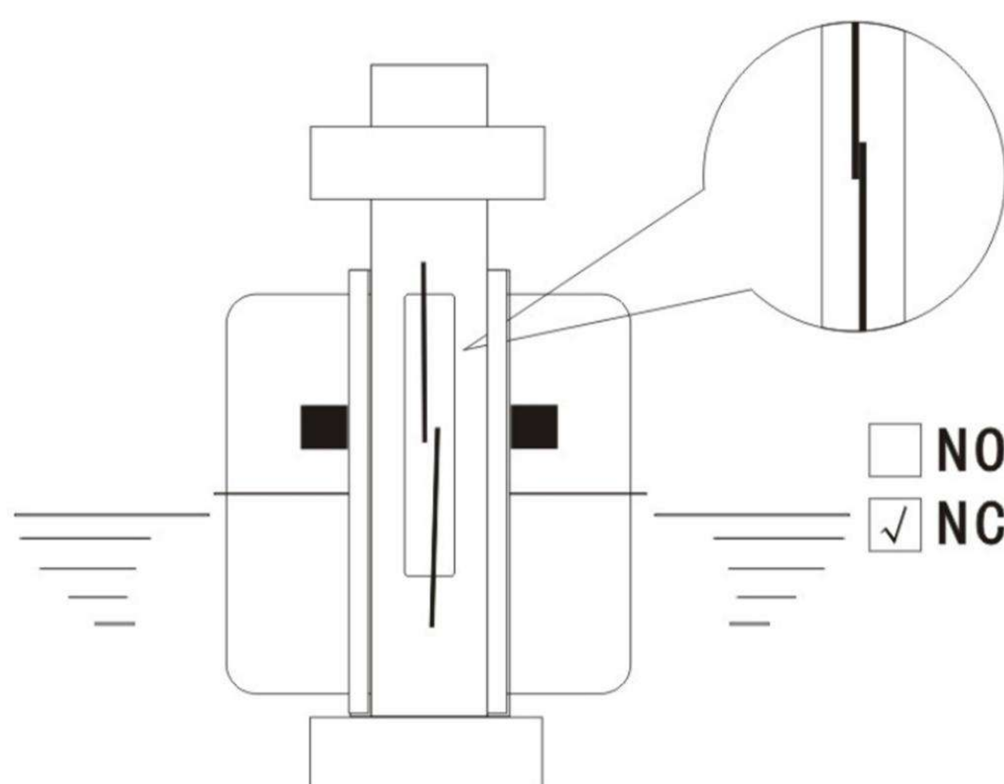
■ 常闭 (N.C) 当液位上升时磁簧开关不导通 Normally closed, when the liquid level rises the reed does not conduct
