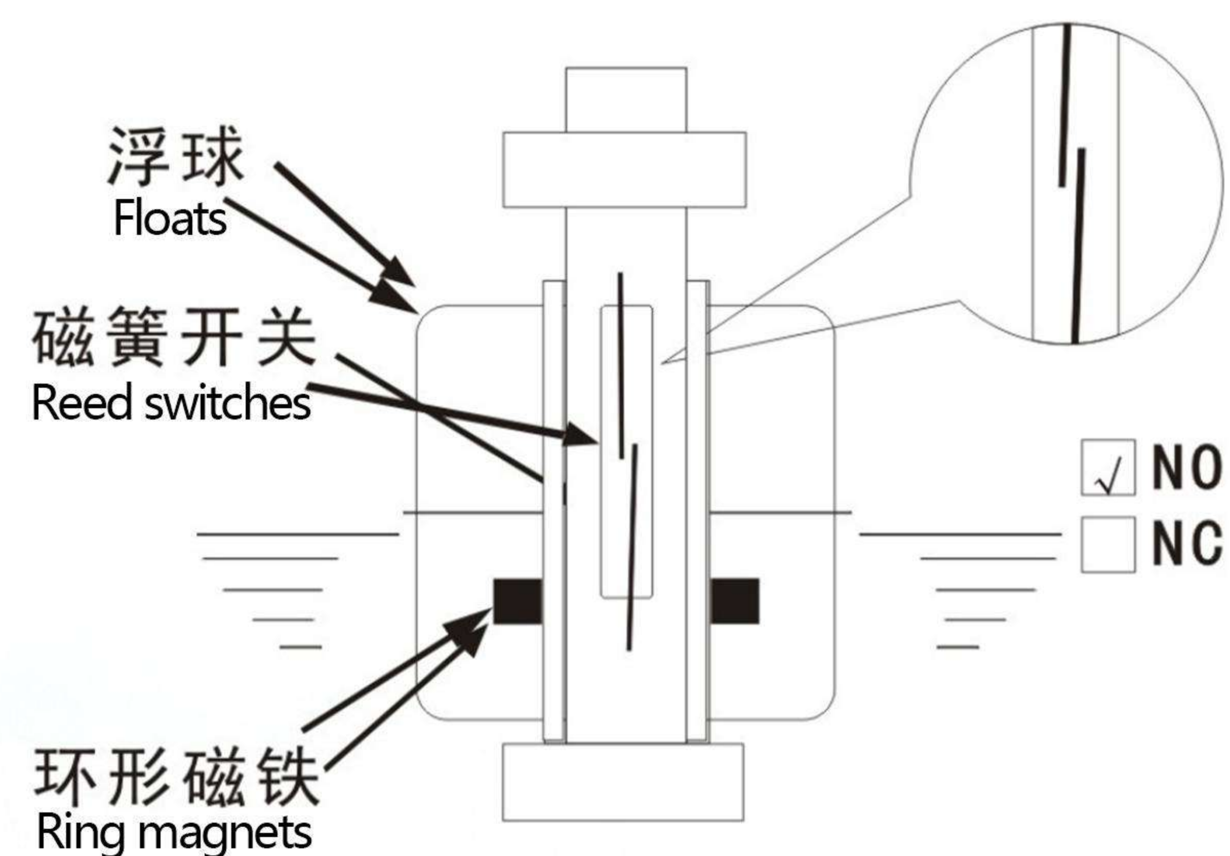
■ 常开 (N.O) 当液位上升时磁簧开关导通 Normally open, when the liquid level rises the reed conductive
