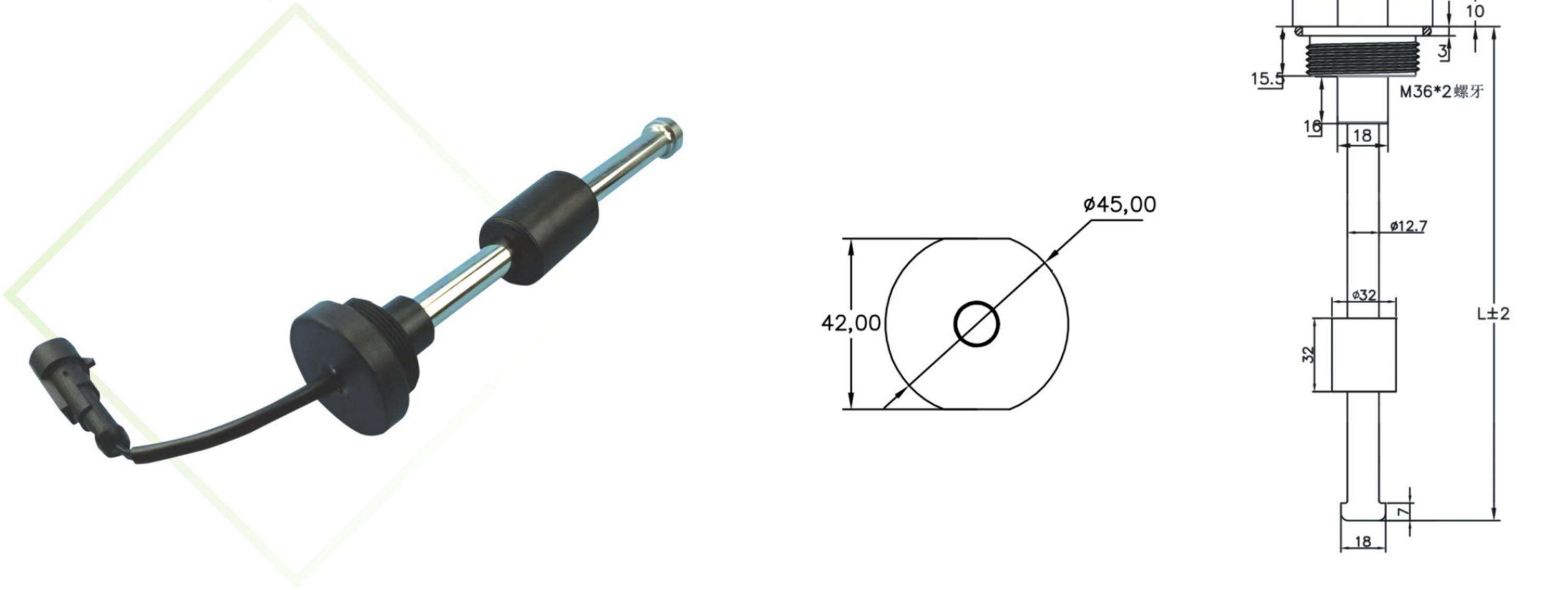
塑料液位传感器选型参考 P.P level sensor selection reference
