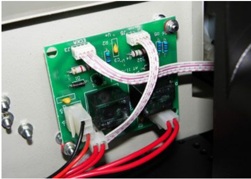
3. Imported Omron components. Put the circuit control board & the total power and power of thread plug structure separate.
