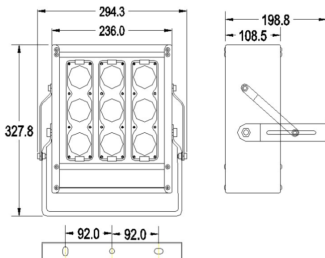
Product Dimension(mm)
