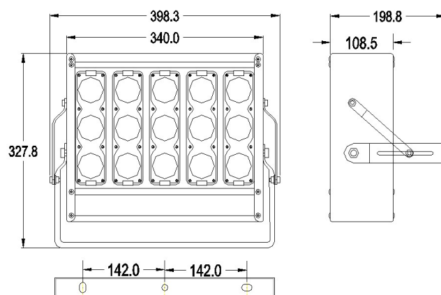
Product Dimension(mm)
