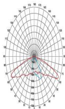
路灯曲线图 illumination angle curve
