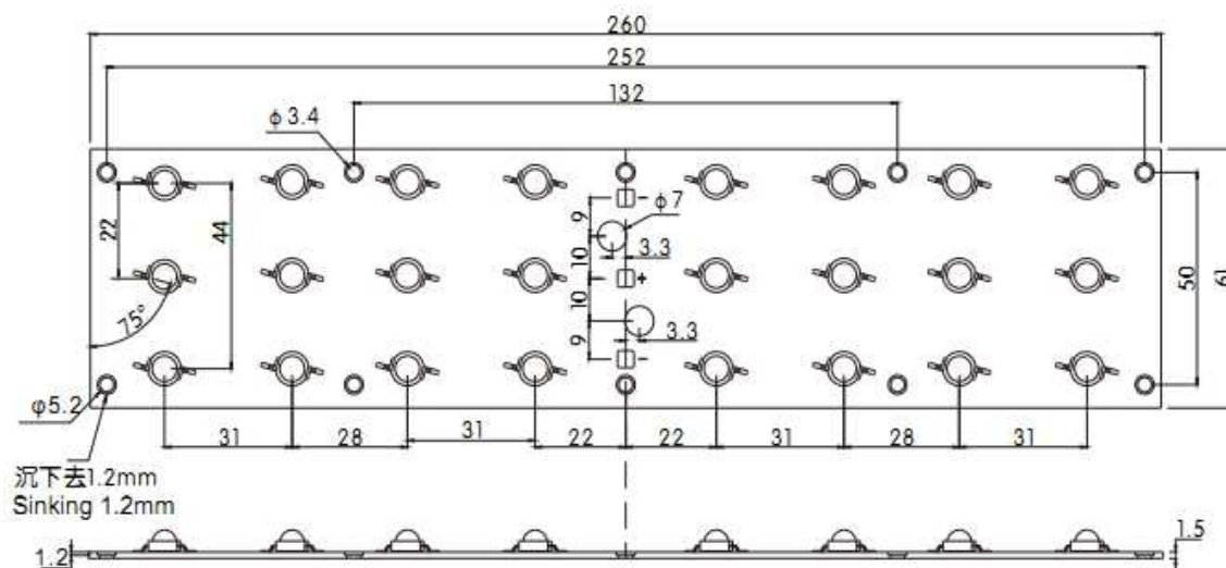
仿流明灯珠铝基板图 Aluminum Plate for Lumiled LED Chip
