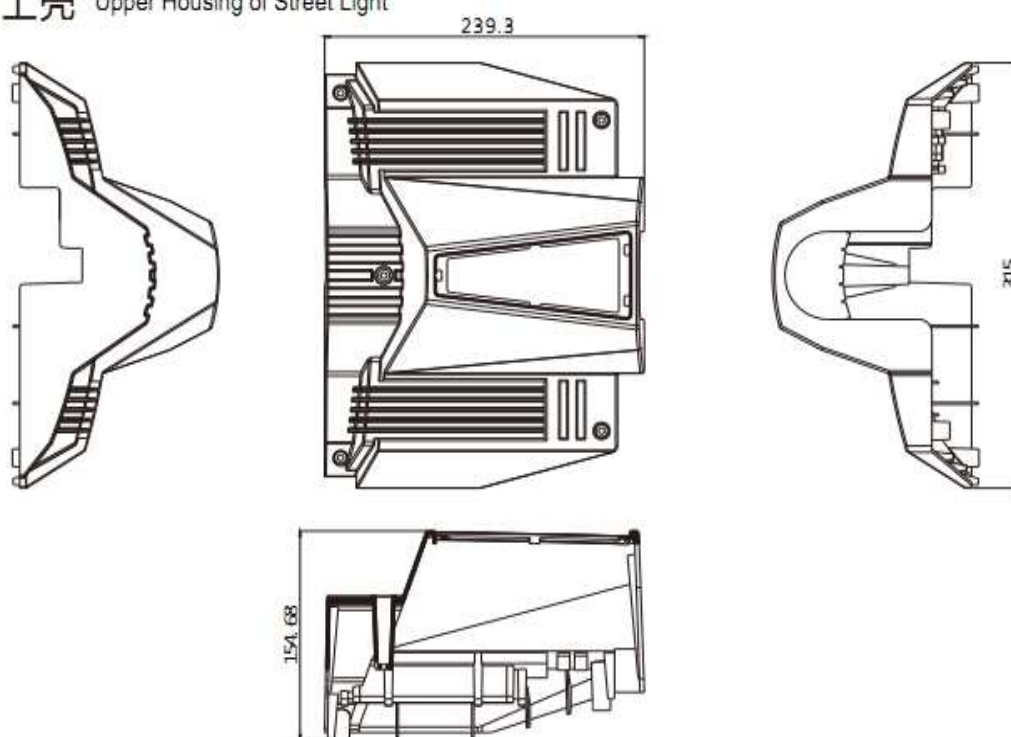
路灯上壳 Upper Housing of Street Light
