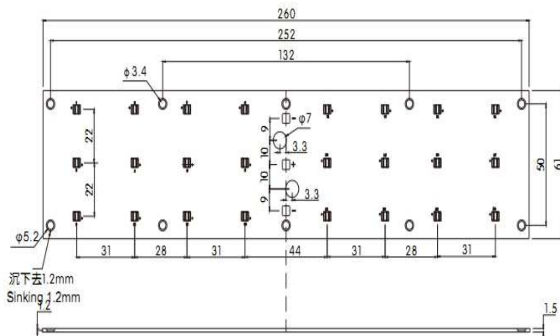
CREE灯珠铝基板图 Aluminum Plate for CREE LED Chip
